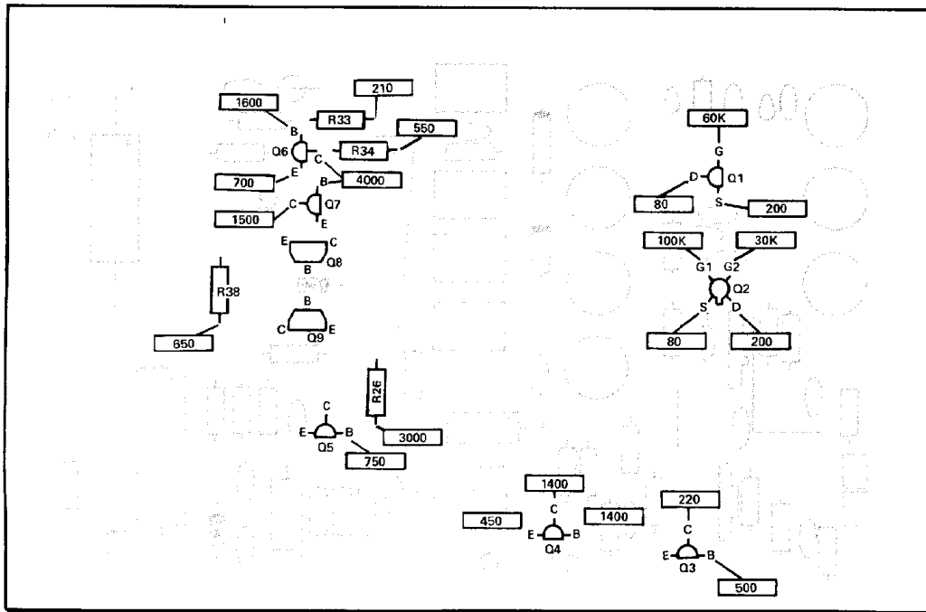
(SHOWN FROM COMPONENT SIDE)
