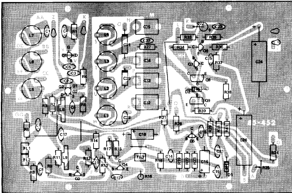
(SHOWN FROM FOIL SIDE)
